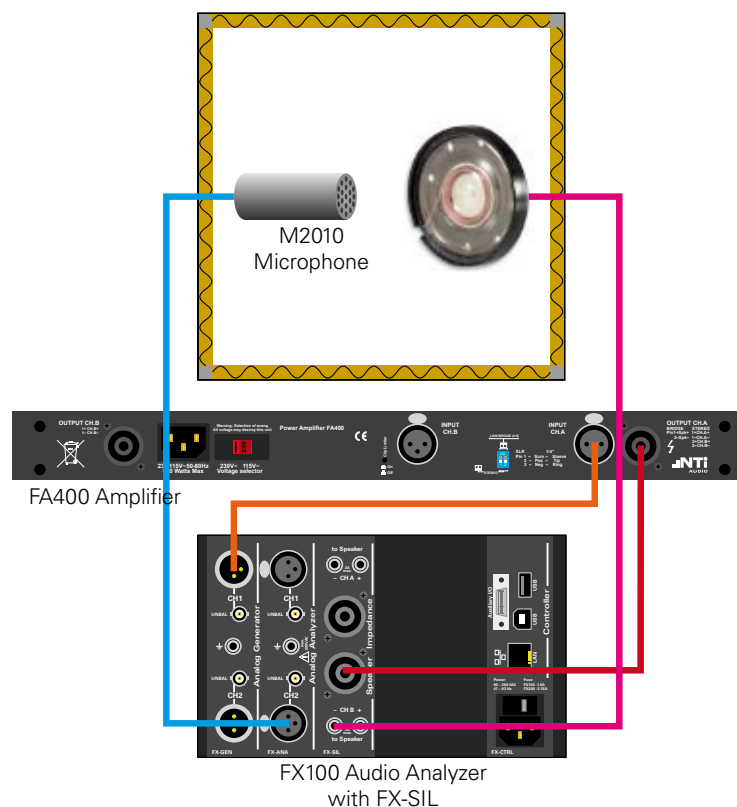
Telecom transducer test setup
