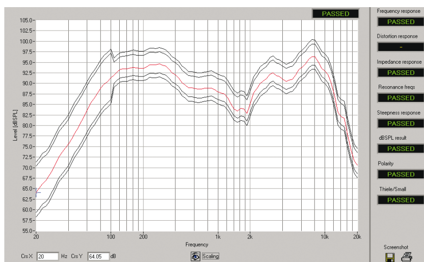
Frequency response measurement with absolute results
