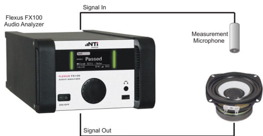
Basic Speaker Test Configuration
