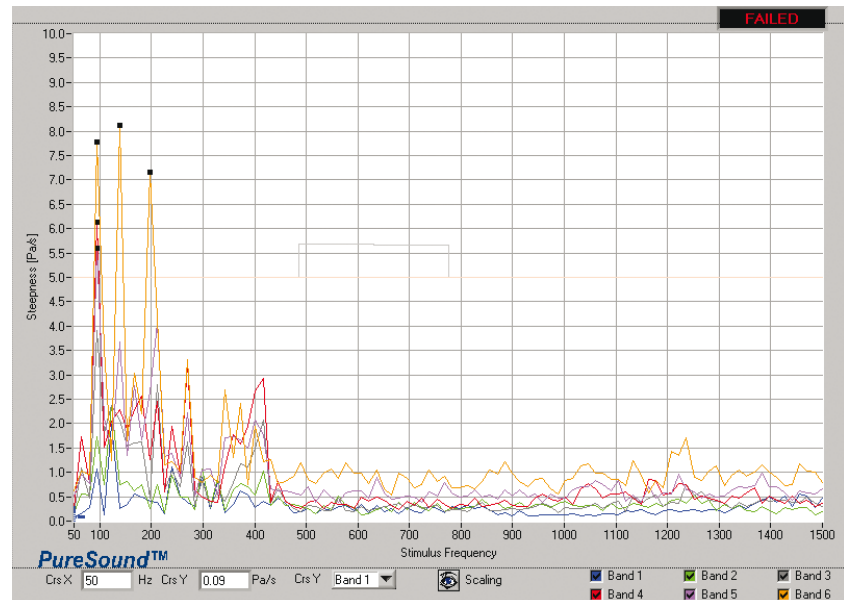
Rub & Buzz analysis: Loose particles
