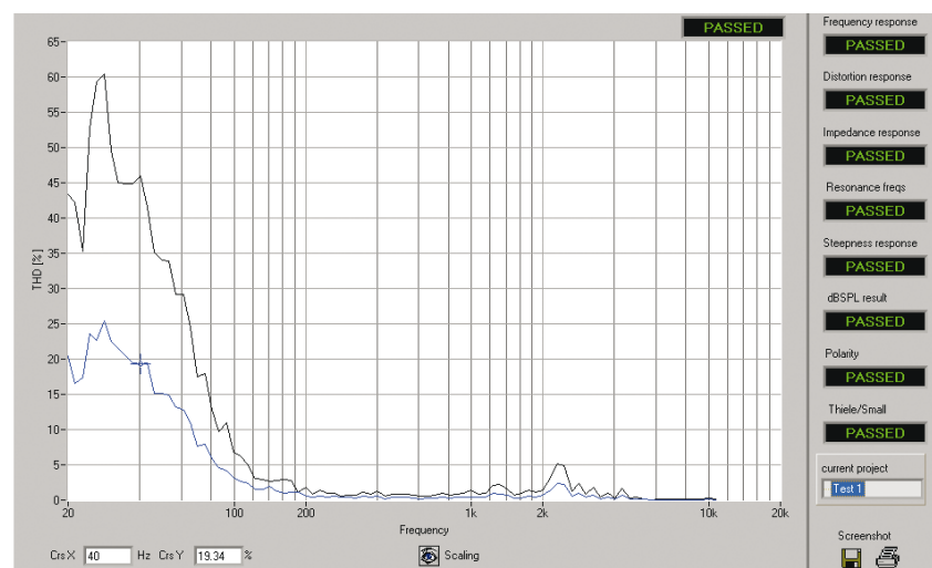
Distortion analysis THD
