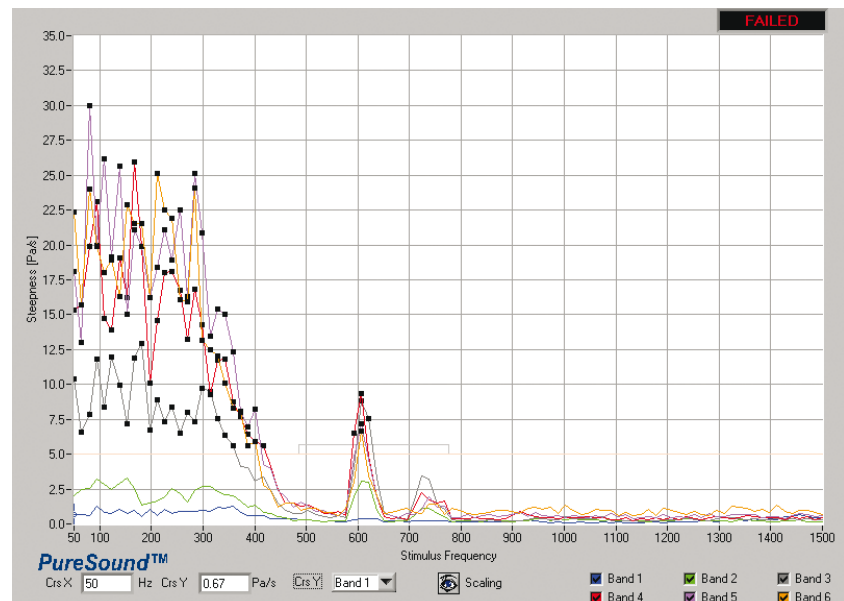
Rub & Buzz analysis: Rubbing voicecoil
