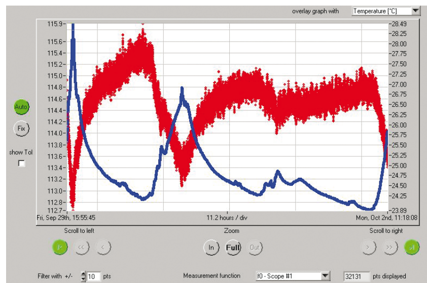
Statistical trend analysis correlated with the environmental temperature
